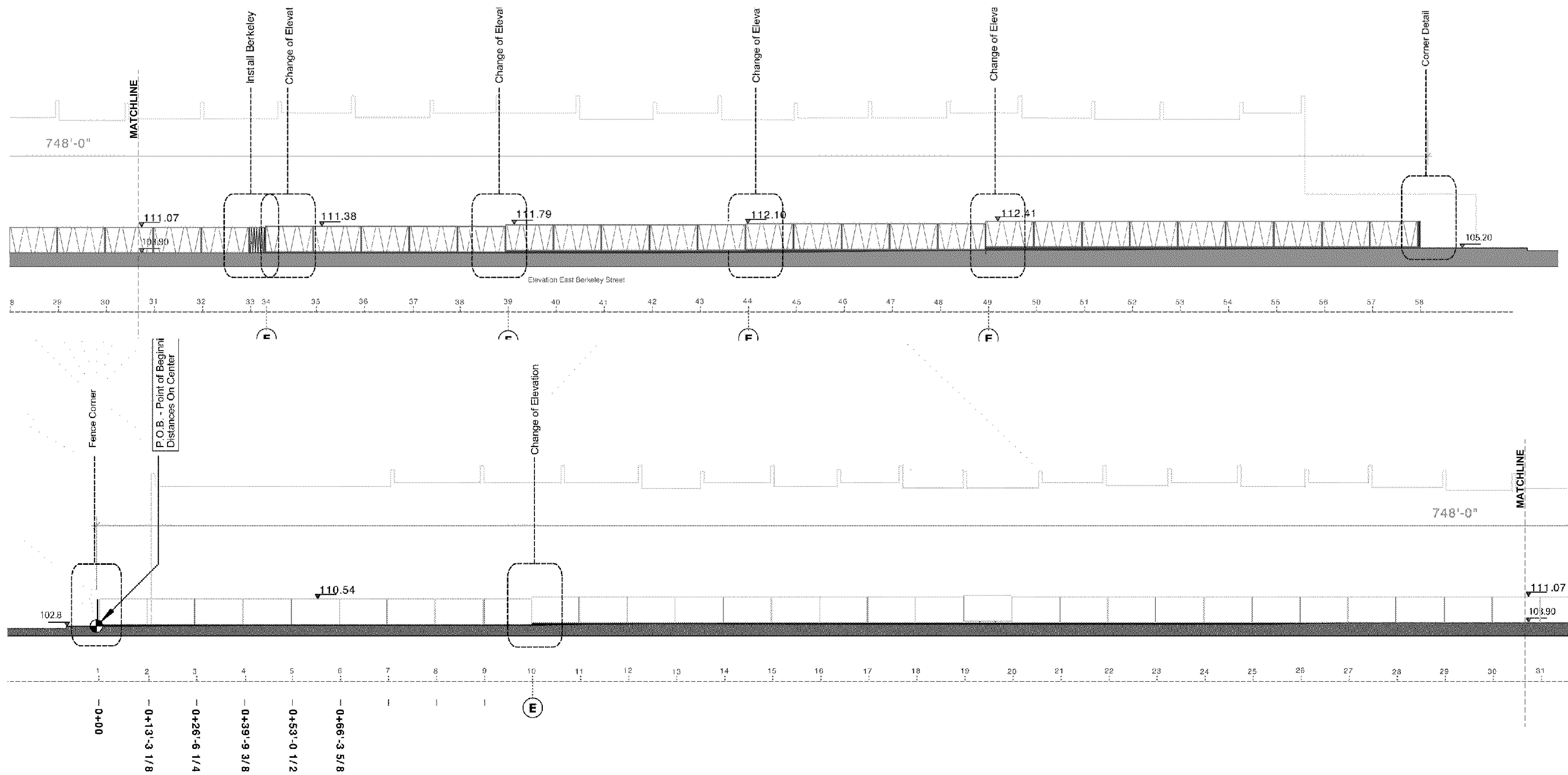
East Berkeley Street Elevation
